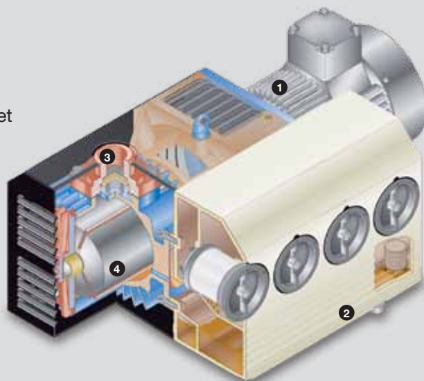
1 Motor | 2 Oil separation | 3 Suction port | 4 Cylinder
